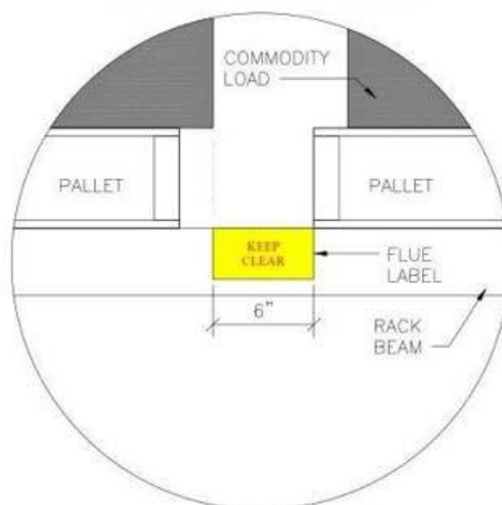
6" TRANSVERSE FLUE LABEL BETWEEN PALLET LOADS
