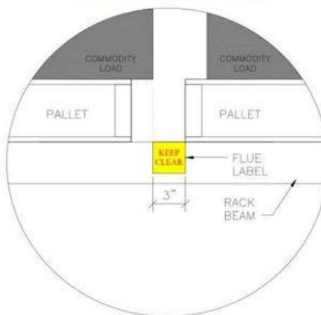
3" TRANSVERSE FLUE LABEL BETWEEN PALLET LOADS
