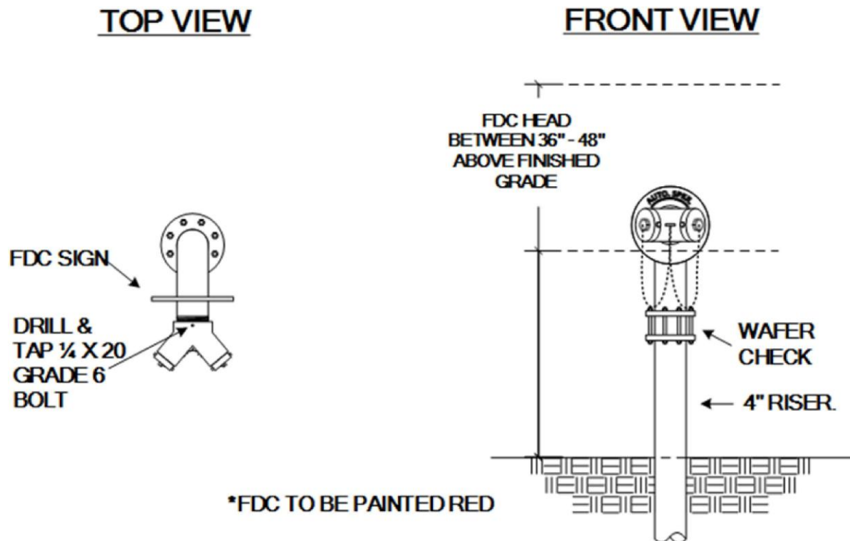
DIAGRAM F-4.2: SINGLE 4" X 2 1/2" X 2 1/2" FDC DETAIL
