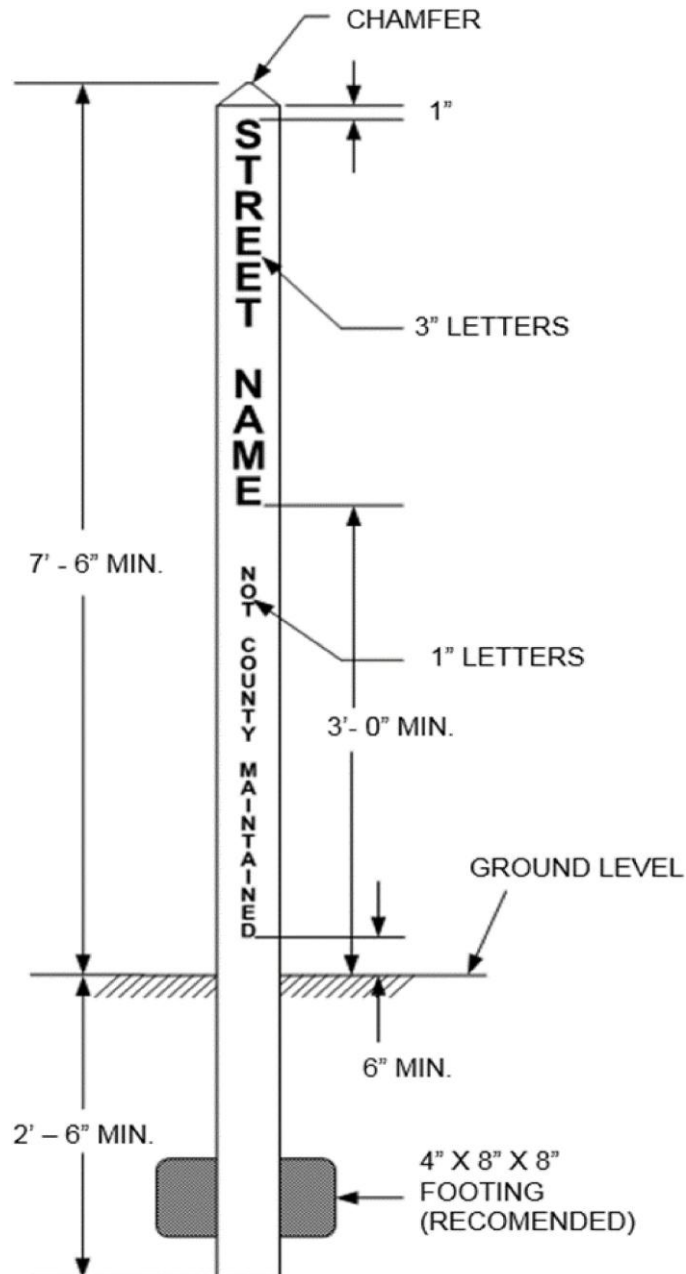
DIAGRAM B-1.2: STREET SIGN POST
